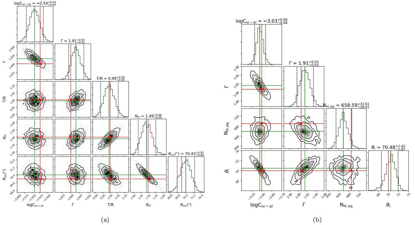
Figure 1: Contour plots for MYTORUS, MCT and HCT regimes respectively
