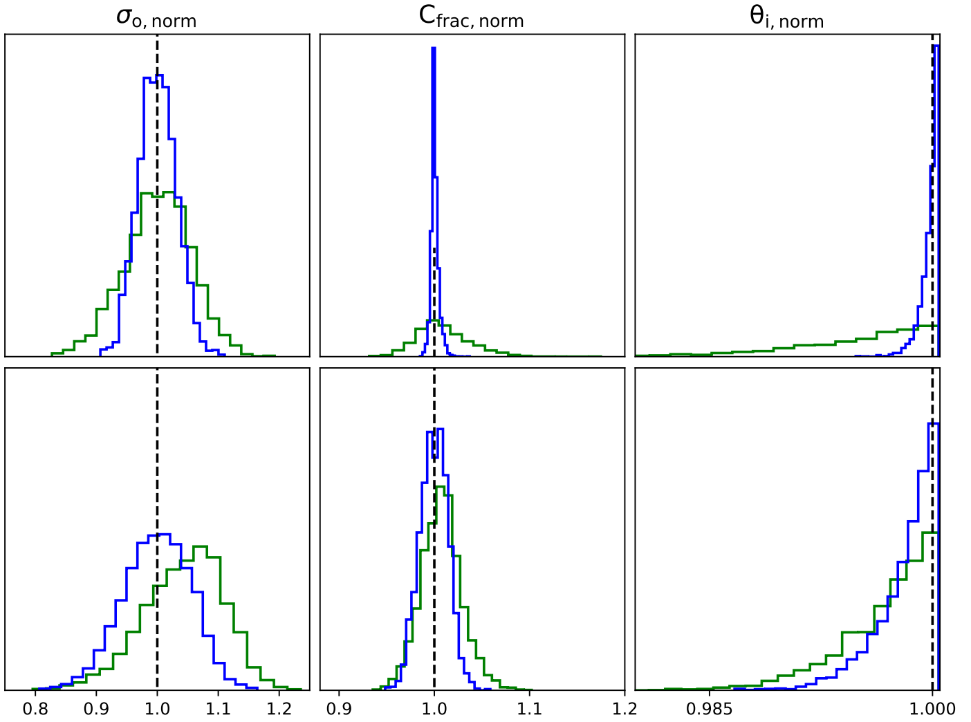
Figure 5: Plots for the in the upper panel are for the case M_{UXCL} \rightarrow D_{CTOR} and the lower panel for the case M_{UXCL} \rightarrow D_{BOR} in the HCT regime.
