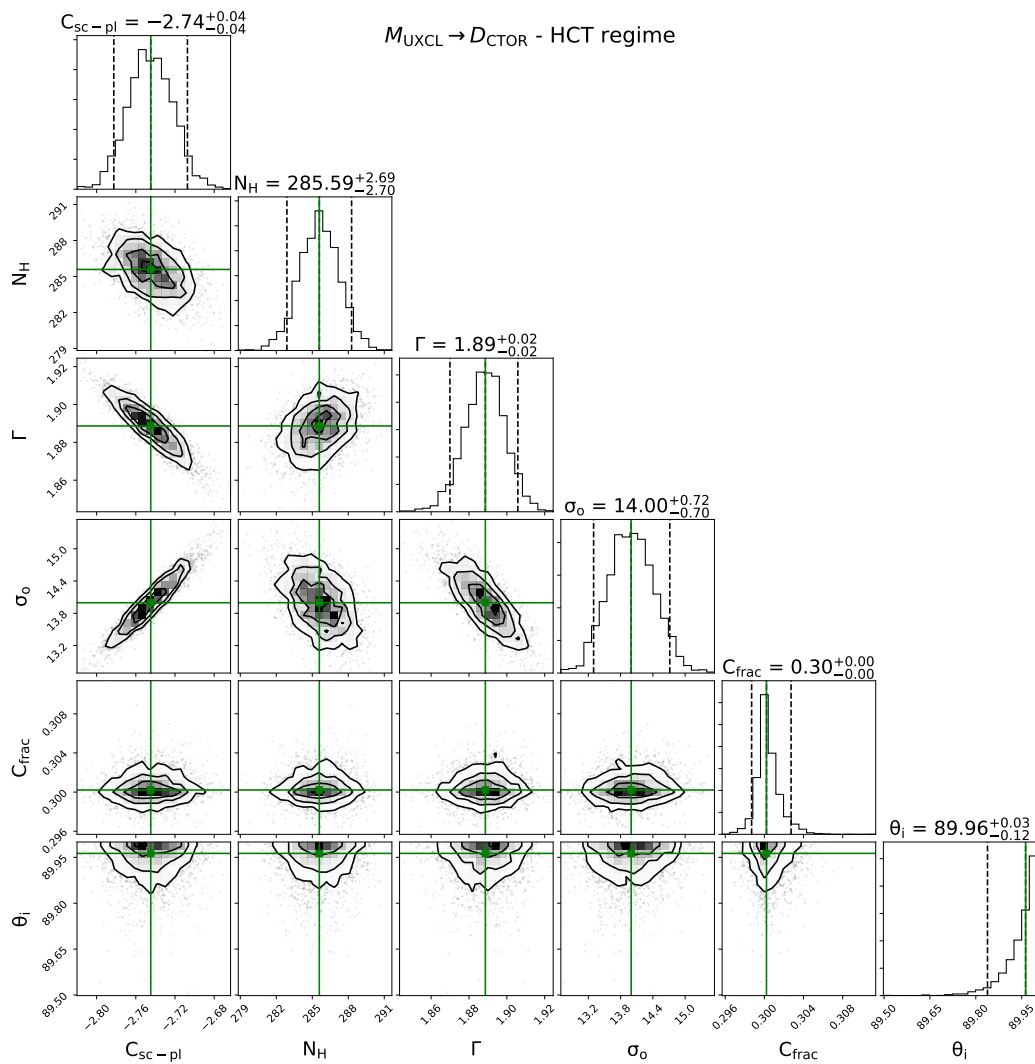
Figure 1: Contours for M_{\text{UXCL}} \rightarrow D_{\text{CTOR}} analysis in the HCT regime, with N_{\text{H,los}} = 500 as input.
