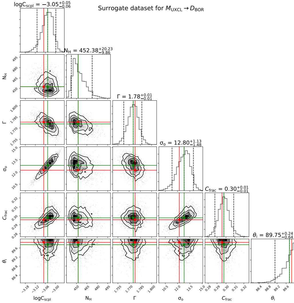
Figure 4: Surrogate dataset for the M_{\text{UXCL}} \rightarrow D_{\text{BOR}} CM fits
