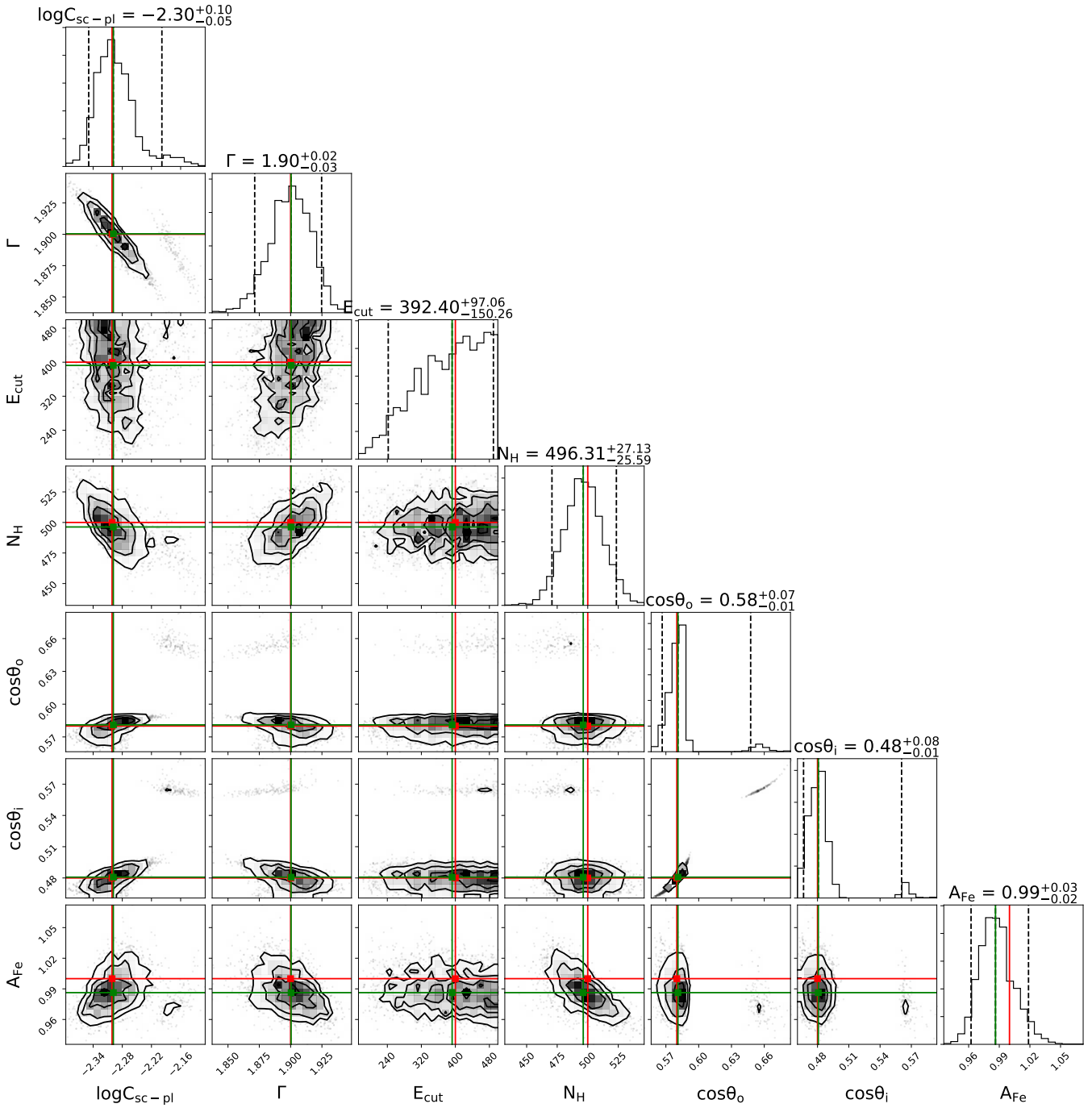
Figure 2: Contours for BORUS IM analysis in the HCT regime with a stronger scattered power law (HCT-0), with N_H = 500 as input, HCT-0
