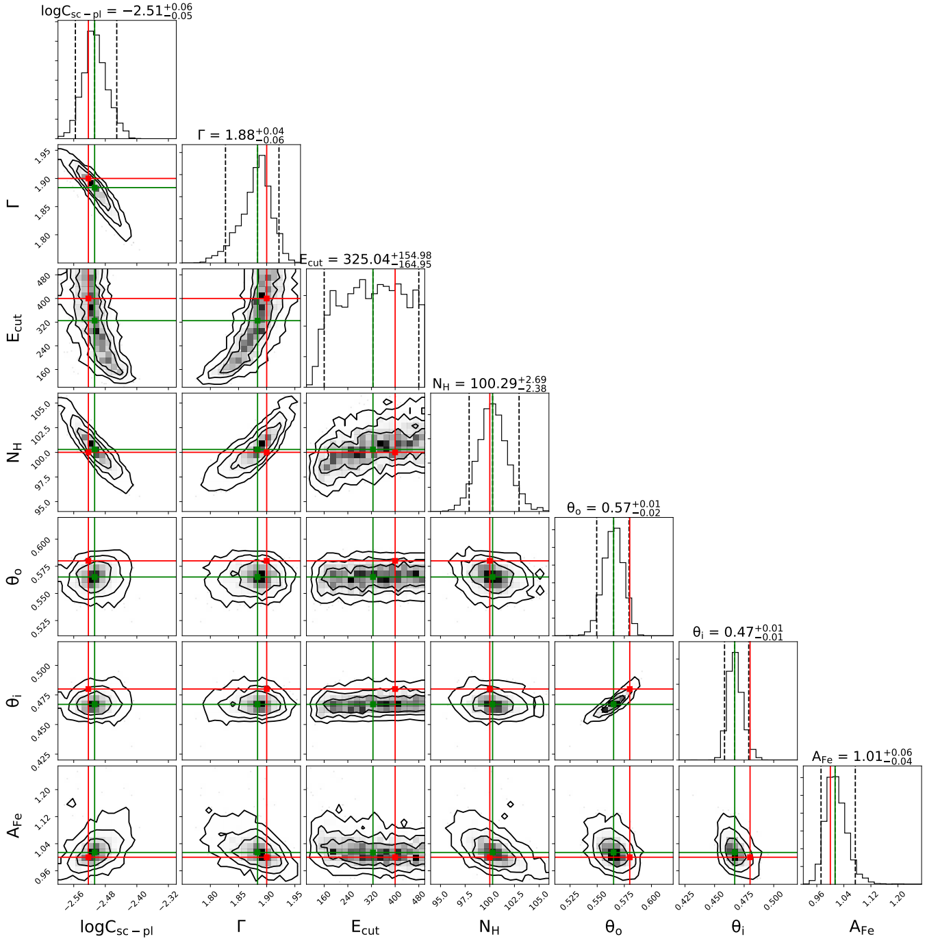
Figure 1: Contours for BORUS IM analysis in the MCT regime, with N_H = 100 as input.
