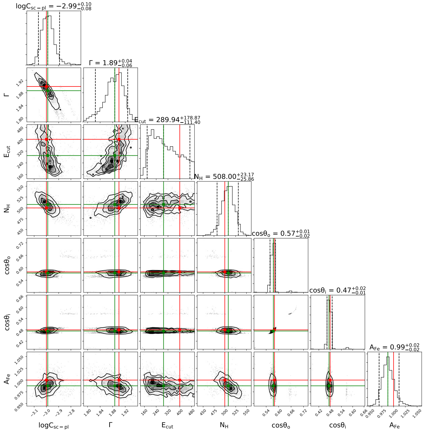
Figure 3: Contours for BORUS IM analysis in the HCT regime, with N_H = 500 as input, (HCT-1)
