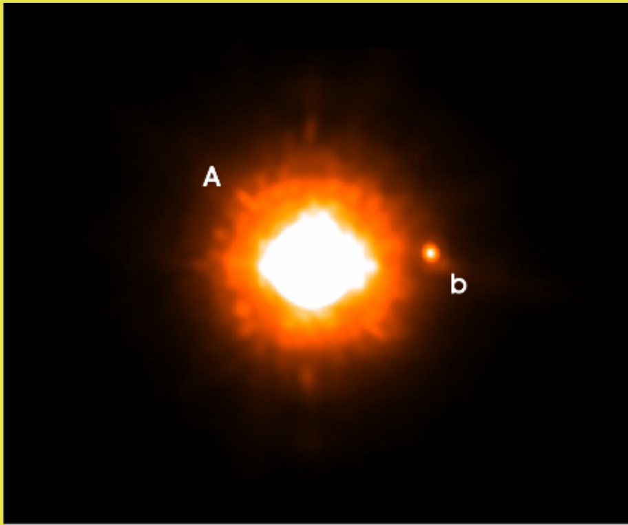
The Sub-Stellar Companion to GQ Lupi (NACO/VLT)
