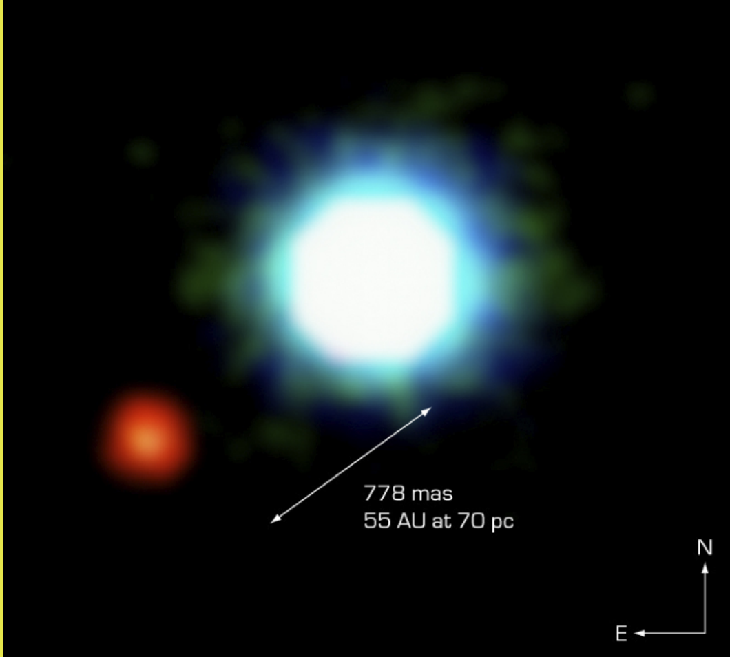
The Brown Dwarf 2M1207 and its Planetary Companion (VLT/NACO)
