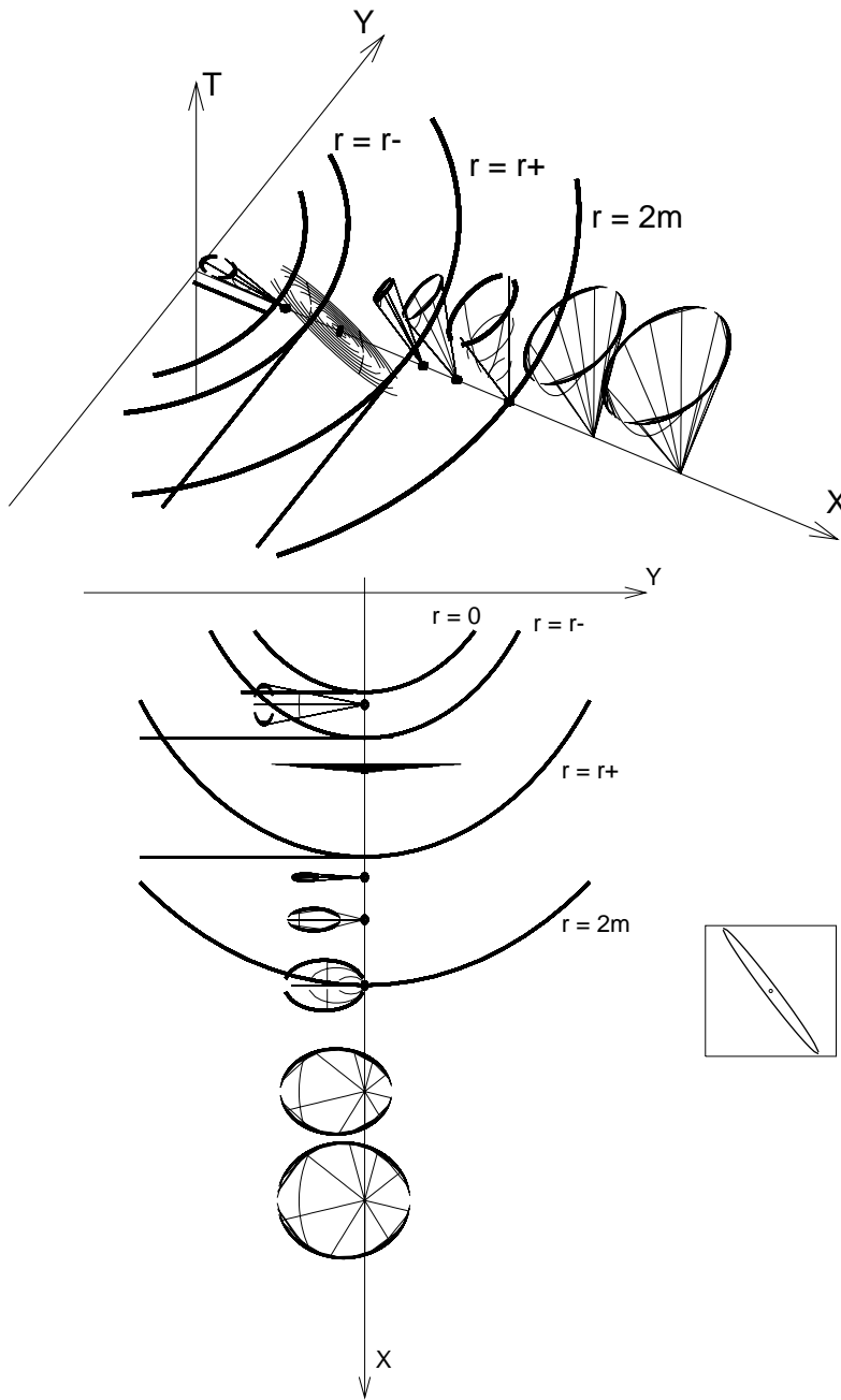
Figure 1: Light cones in the vicinity of a rotating black hole. Want more explanation? See my book “An introduction to general relativity and cosmology”, Fig. 20.6 on p. 463.
